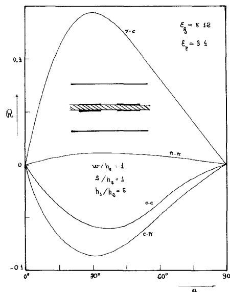
Fig. 6. Variation of the R -parameters in the broadside edge-coupled microstrips with an inverted substrate of boron nitride, as functions of the tilting angle of the substrate ( \epsilon_f^* = 5.12 , \epsilon_r^* = 3.4 ).
