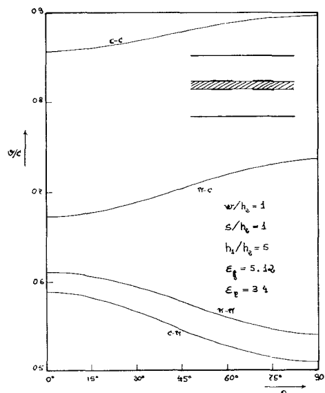
Fig. 5. Variation of the normalized phase velocities in the broadside edge-coupled microstrips with an inverted substrate of boron nitride, as functions of the tilting angle ( \epsilon_f^* = 5.12 , \epsilon_r^* = 3.4 ).
